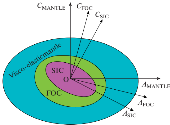
Fig. 1. Cross-section of the Moon along its axis of rotation. The fluid outer core (FOC) and the solid inner core (SIC) are axisymmetric: A_{\text{MANTLE}} = B_{\text{MANTLE}} , A_{\text{FOC}} = B_{\text{FOC}} , A_{\text{SIC}} = B_{\text{SIC}} —are the equatorial moments of inertia for the mantle and both nuclei. The moments C_{\text{MANTLE}} , C_{\text{FOC}} , C_{\text{SIC}} —are the maximum moments of inertia.
