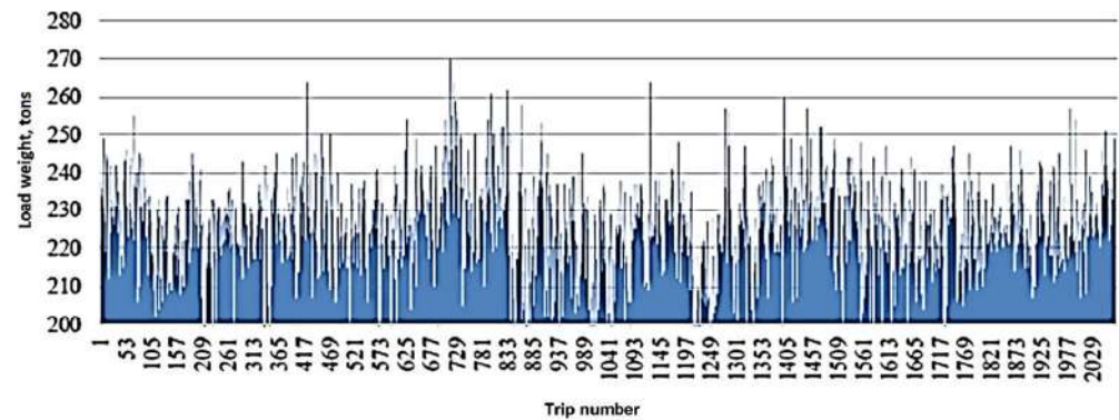
Figure 5. Data on the BELAZ 75306 dump truck operation depending on the trip number.
